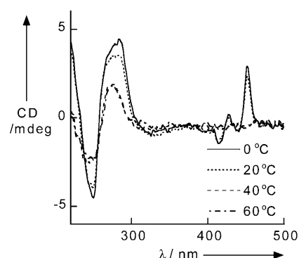
Figure 3. CD spectra of ODN7/C2 at various temperatures. Solution conditions are as follows: [ ODN7 ] = 1.0 \mu M, [ C2 ] = 1.2 \mu M, [NaCl] = 100 mM, pH 7.0 (10 mM phosphate buffer).
