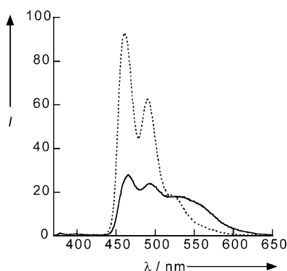
Figure 4. Fluorescence emission spectra of ODN7/C1 (—) and ODN7/C2 (.....) at 20°C. The excitation wavelength was 345 nm. Solution conditions are as follows: [ODN7] = 1.0 \mu\text{M} , [Cn] = 1.2 \mu\text{M} , [NaCl] = 100 mM, pH 7.0 (10 mM phosphate buffer).
