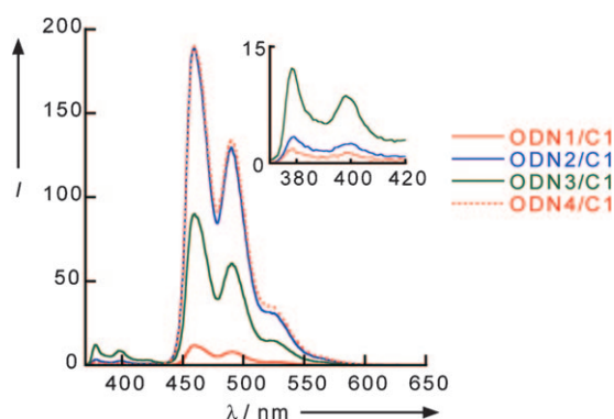
Figure 1. Fluorescence emission spectra of ODN1/C1–ODN4/C1 at 0°C. Spectra at 370–420 nm are magnified in the inset. The excitation wavelength was 345 nm. The solution conditions are as follows: [\text{ODN}] = 1.0 \mu\text{M} , [\text{C1}] = 1.2 \mu\text{M} , [\text{NaCl}] = 100 \text{ mM} , pH 7.0 (10 mM phosphate buffer).
