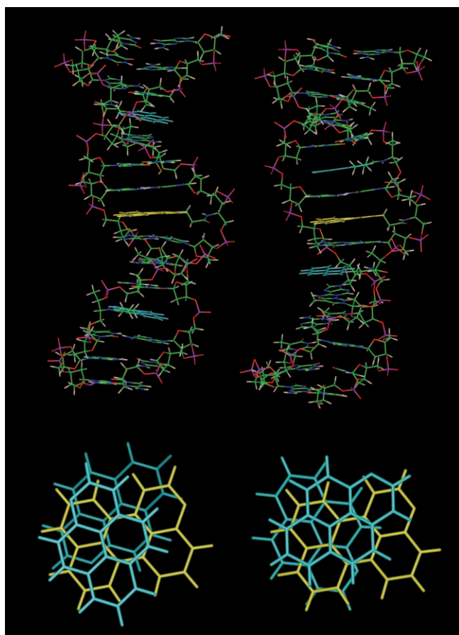
Figure 5. Energy-minimized structures of ODN3/C1 (left side) and ODN2/C1 (right side). The relative orientations of the chromophores are shown at the bottom. Pyrene and perylene moieties are coloured in blue and yellow, respectively.
