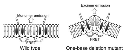
Scheme 2. Schematic illustration of the design of the FRET probe.
