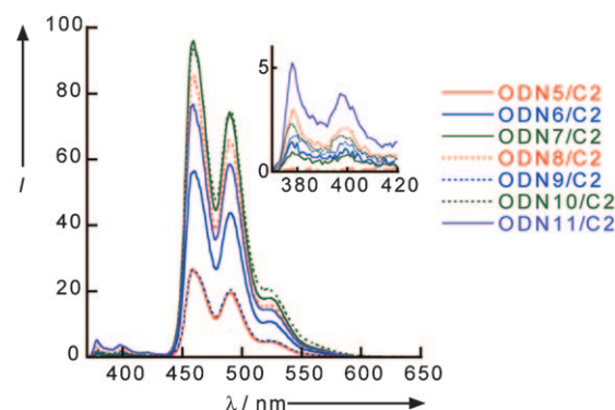
Figure 2. Fluorescence emission spectra of ODN5/C2–ODN11/C2 at 0°C. The excitation wavelength was 345 nm. Spectra at 370–420 nm are magnified in the inset. Solution conditions are as follows: [\text{ODN}] = 1.0 \mu\text{M} , [\text{C2}] = 1.2 \mu\text{M} , [\text{NaCl}] = 100 \text{ mM} , pH 7.0 (10 mM phosphate buffer).
