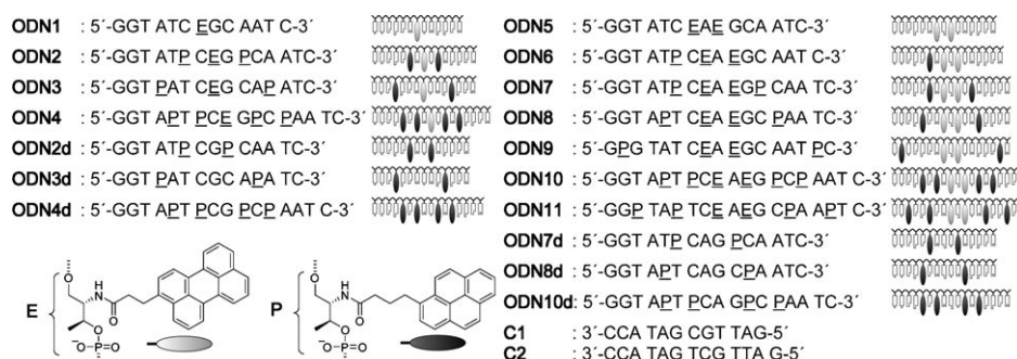
Scheme 1. Sequences of the ODNs synthesized in this study.
